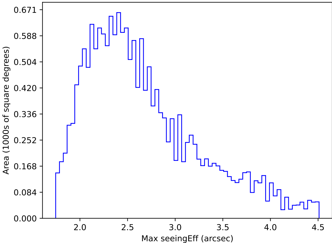
weather_cloudso16v3.4_10yrs WFD g band: Max seeingEff
