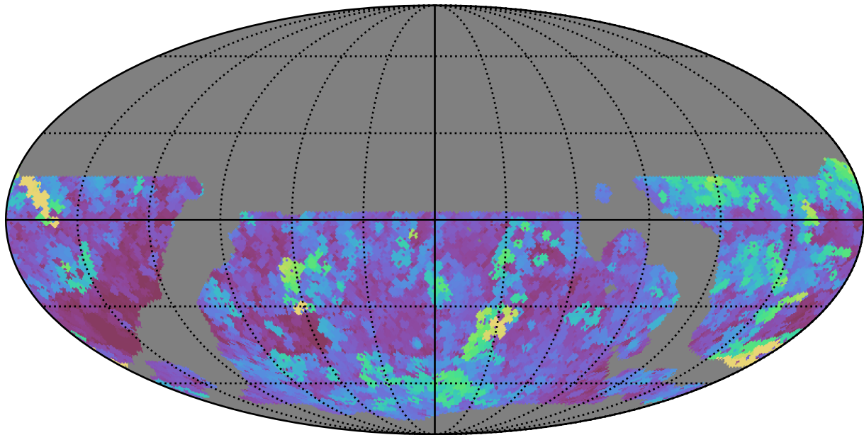
weather_cloudso16v3.4_10yrs WFD all bands: Max seeingEff
