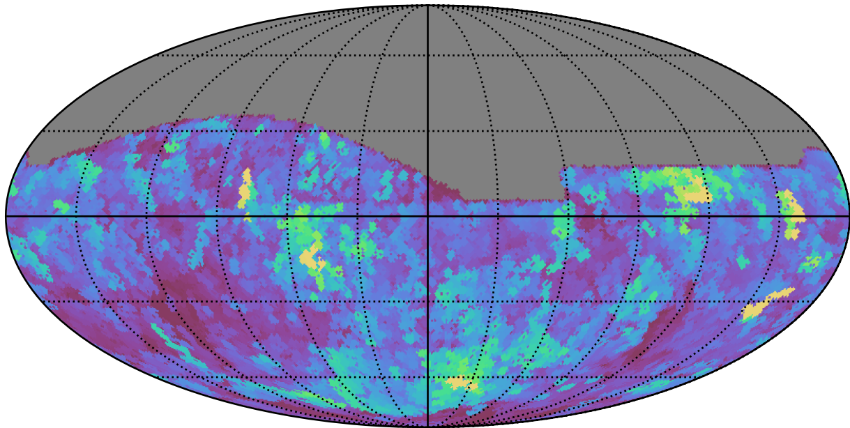
weather_cloudso16v3.4_10yrs All sky z band: Max seeingEff
