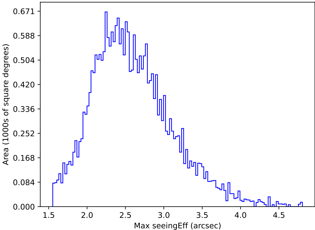
weather_cloudso16v3.4_10yrs All sky z band: Max seeingEff
