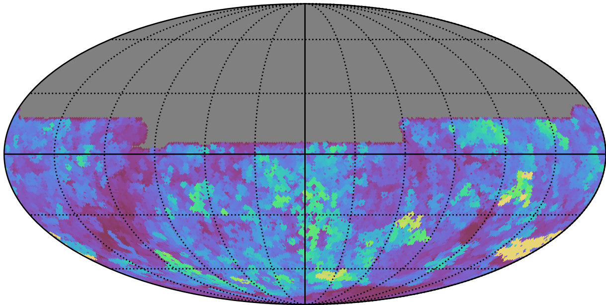
weather_cloudso16v3.4_10yrs All sky y band: Max seeingEff
