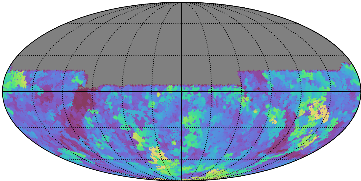
weather_cloudso16v3.4_10yrs All sky u band: Max seeingEff
