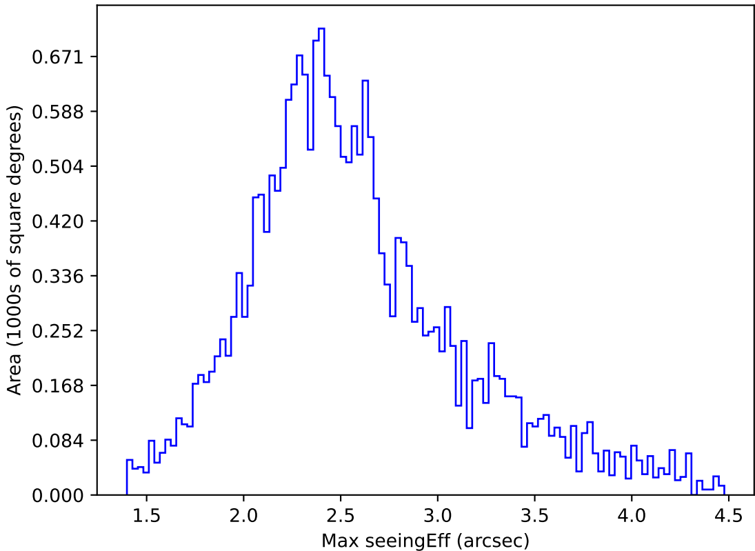
weather_cloudso16v3.4_10yrs All sky u band: Max seeingEff
