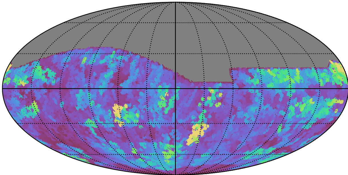
weather_cloudso16v3.4_10yrs All sky r band: Max seeingEff
