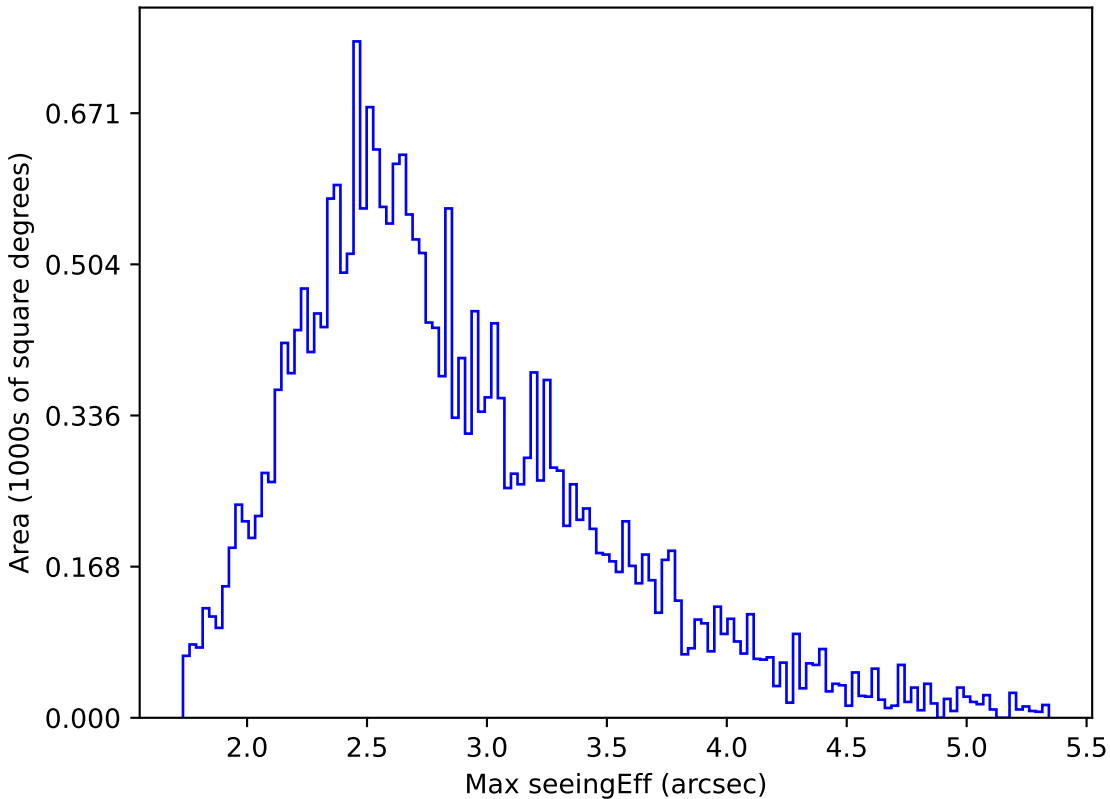
weather_cloudso16v3.4_10yrs All sky r band: Max seeingEff
