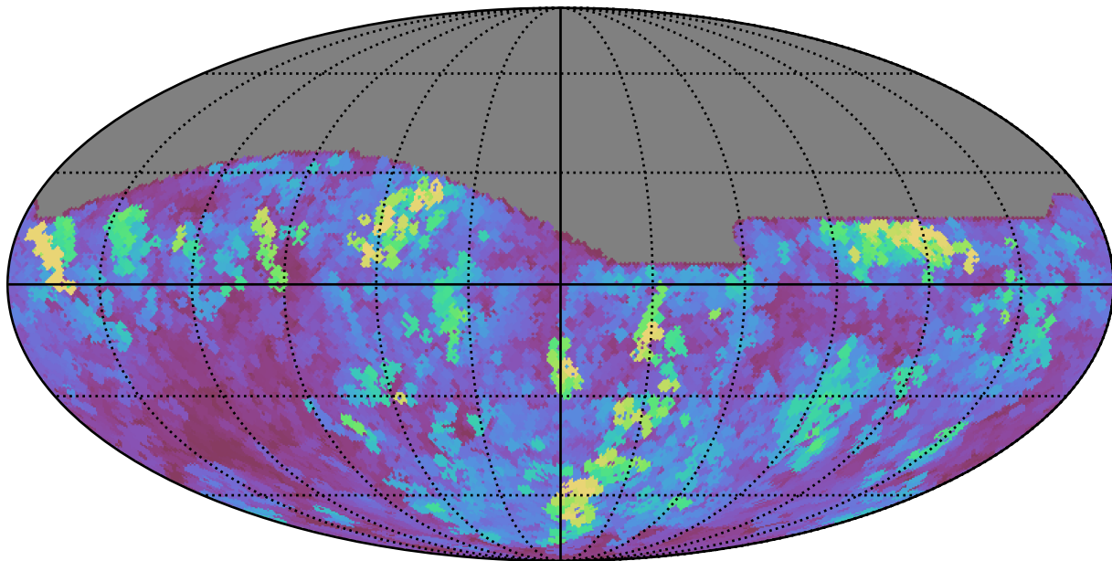
weather_cloudso16v3.4_10yrs All sky i band: Max seeingEff
