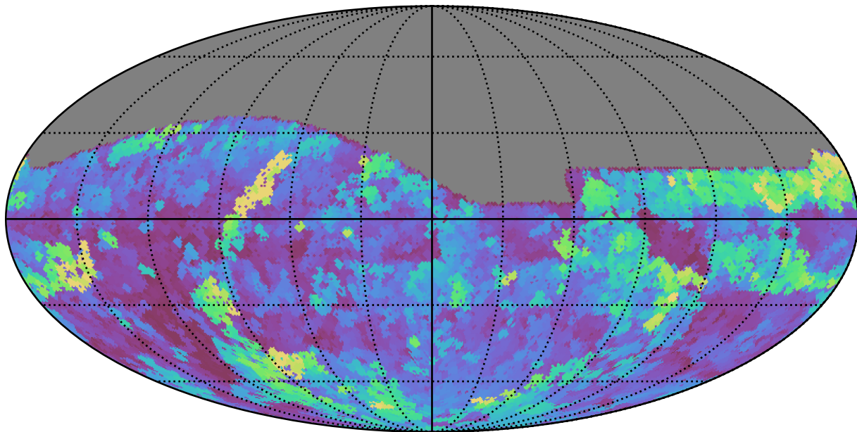
weather_cloudso16v3.4_10yrs All sky g band: Max seeingEff
