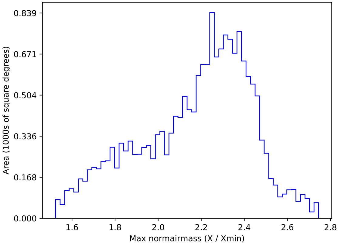
weather_cloudso16v3.4_10yrs WFD r band: Max normairmass
