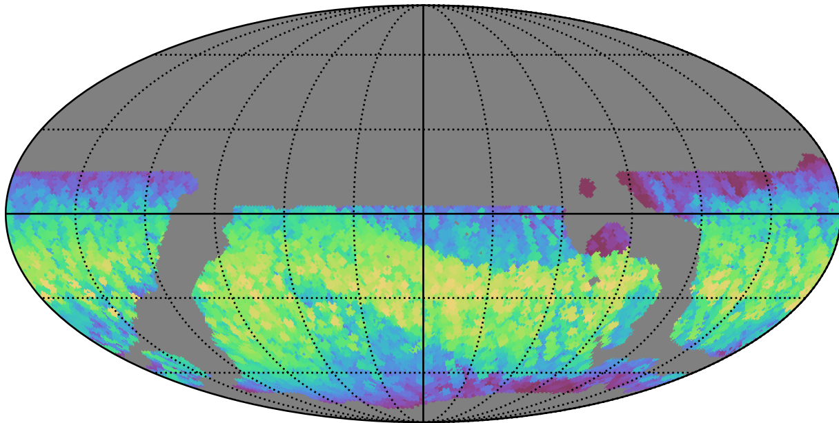
weather_cloudso16v3.4_10yrs WFD all bands: Max normairmass
