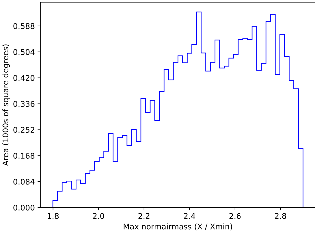
weather_cloudso16v3.4_10yrs WFD all bands: Max normairmass
