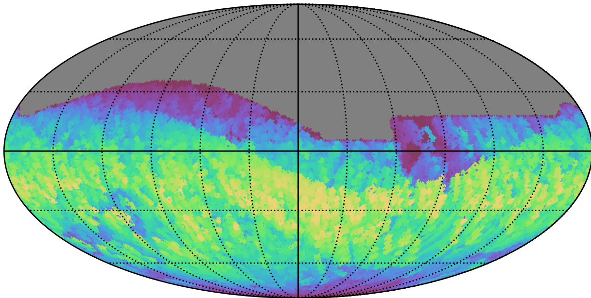
weather_cloudso16v3.4_10yrs All sky z band: Max normairmass
