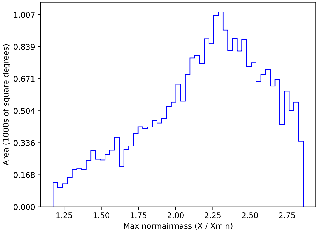
weather_cloudso16v3.4_10yrs All sky z band: Max normairmass
