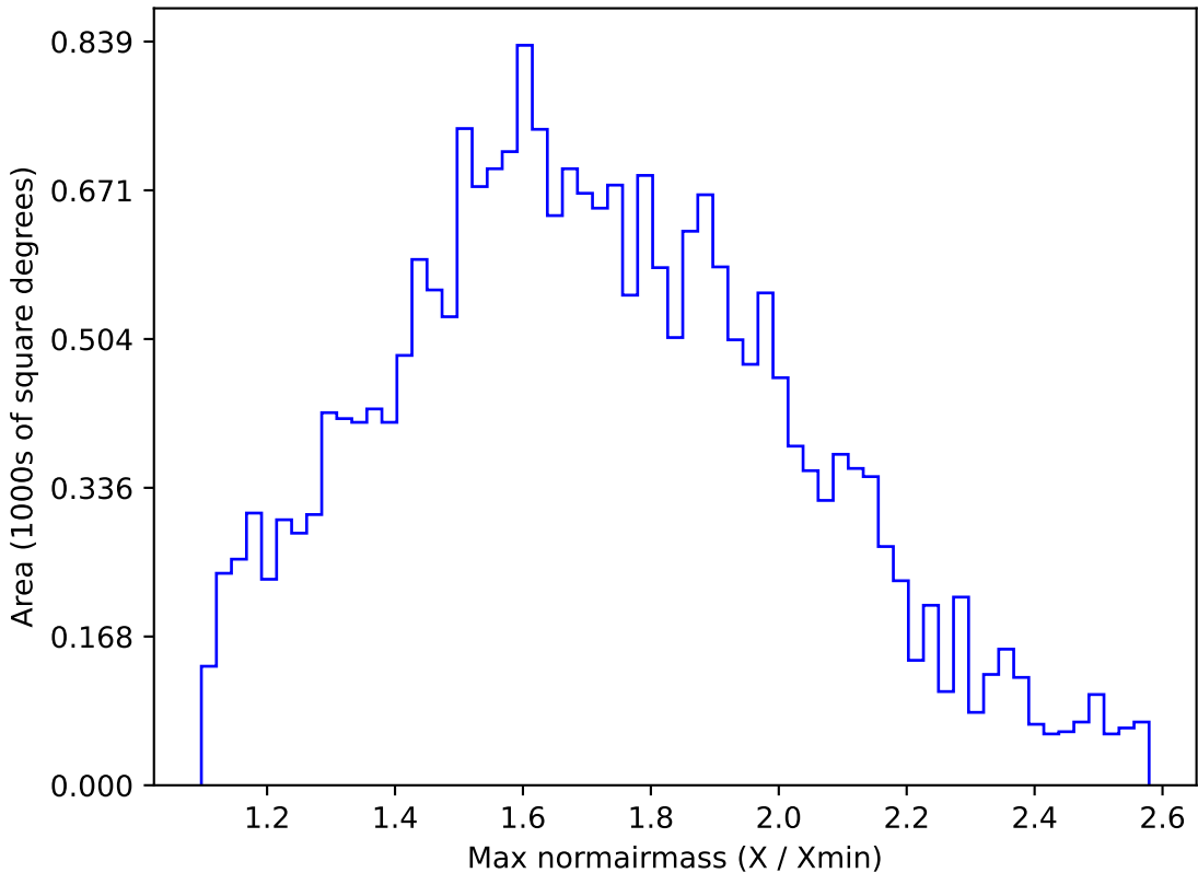
weather_cloudso16v3.4_10yrs All sky u band: Max normairmass
