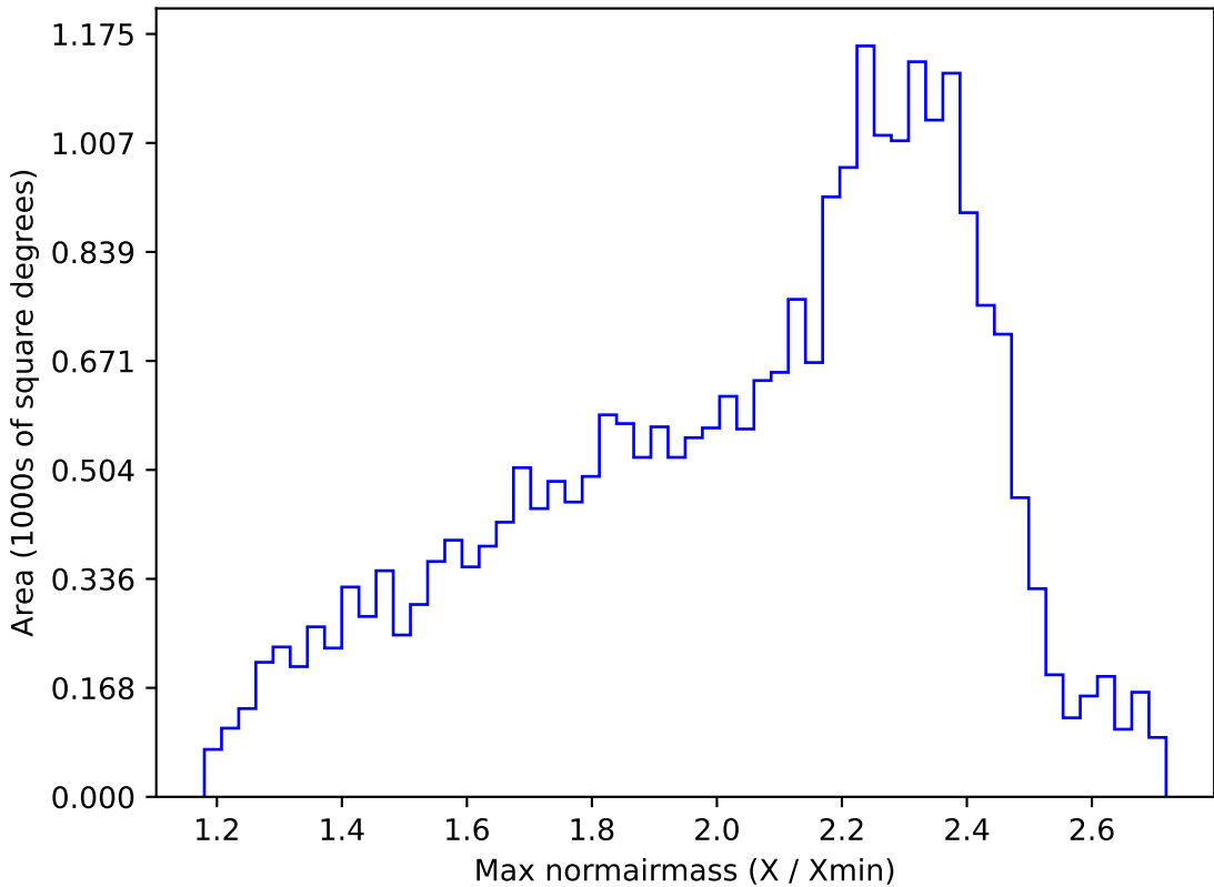
weather_cloudso16v3.4_10yrs All sky r band: Max normairmass
