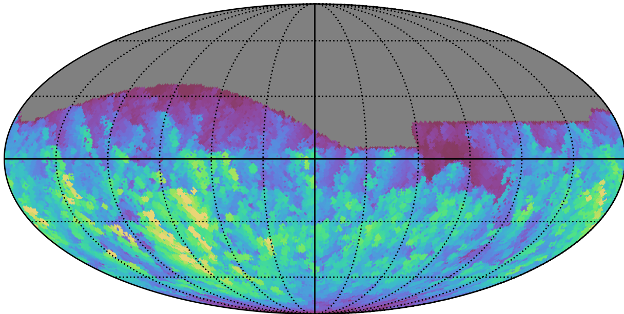
weather_cloudso16v3.4_10yrs All sky g band: Max normairmass
