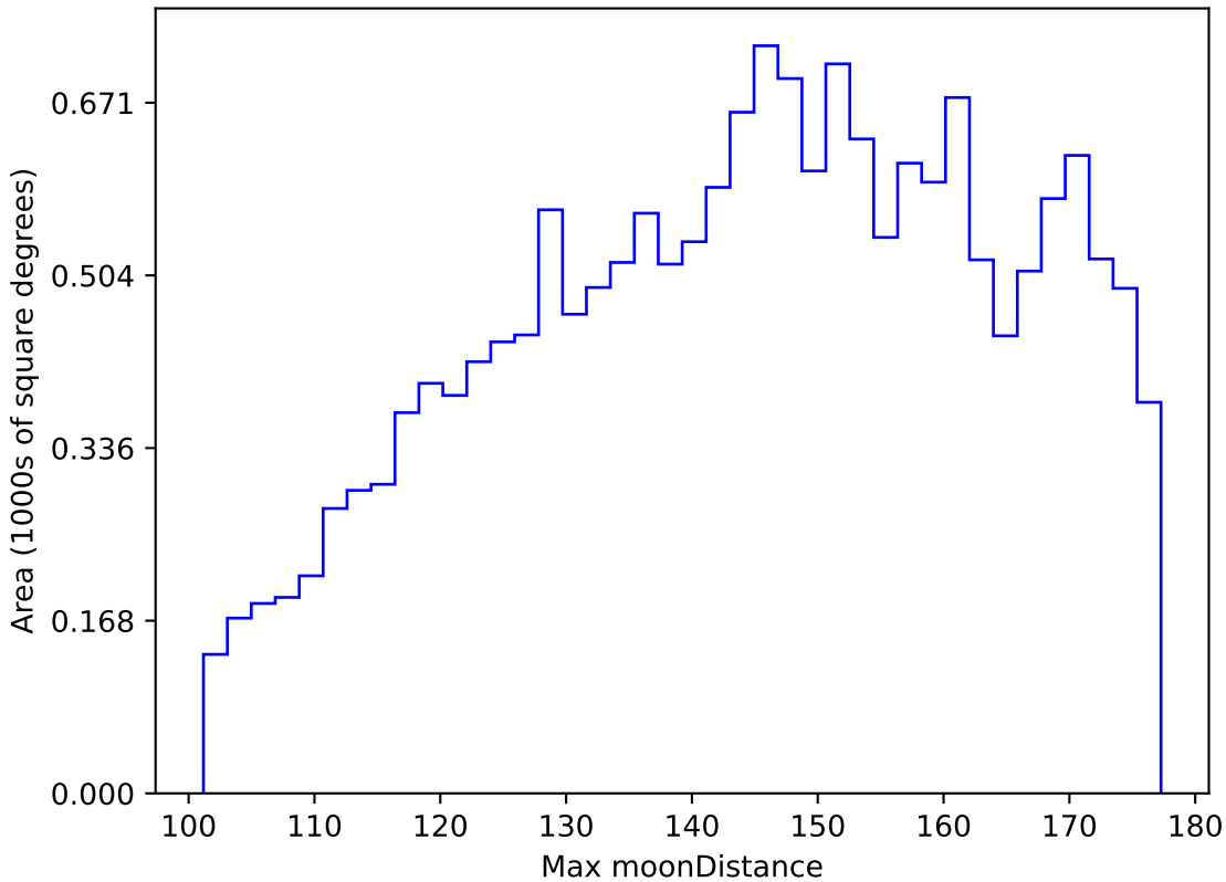
weather_cloudso16v3.4_10yrs WFD y band: Max moonDistance
