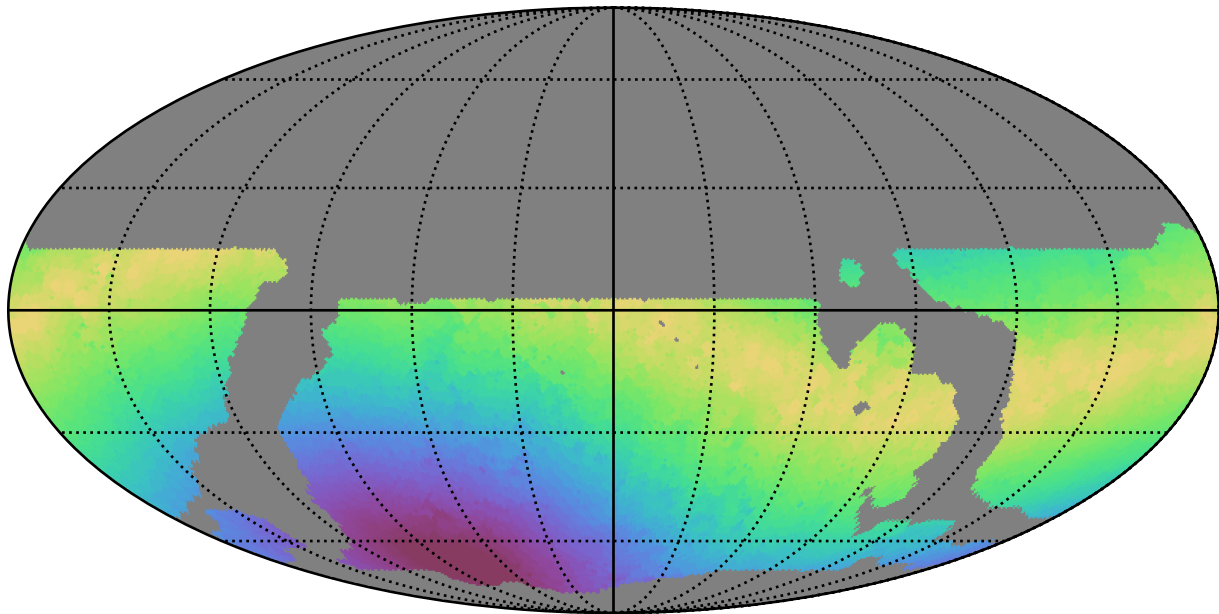
weather_cloudso16v3.4_10yrs WFD u band: Max moonDistance
