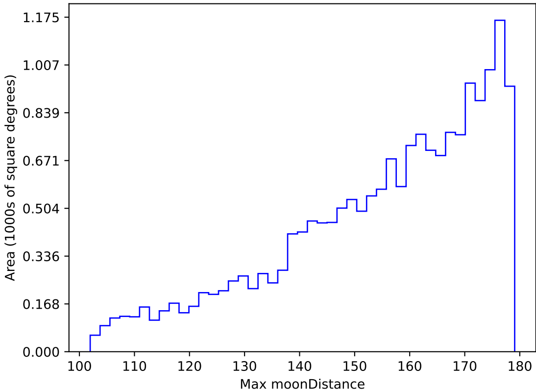
weather_cloudso16v3.4_10yrs WFD u band: Max moonDistance
