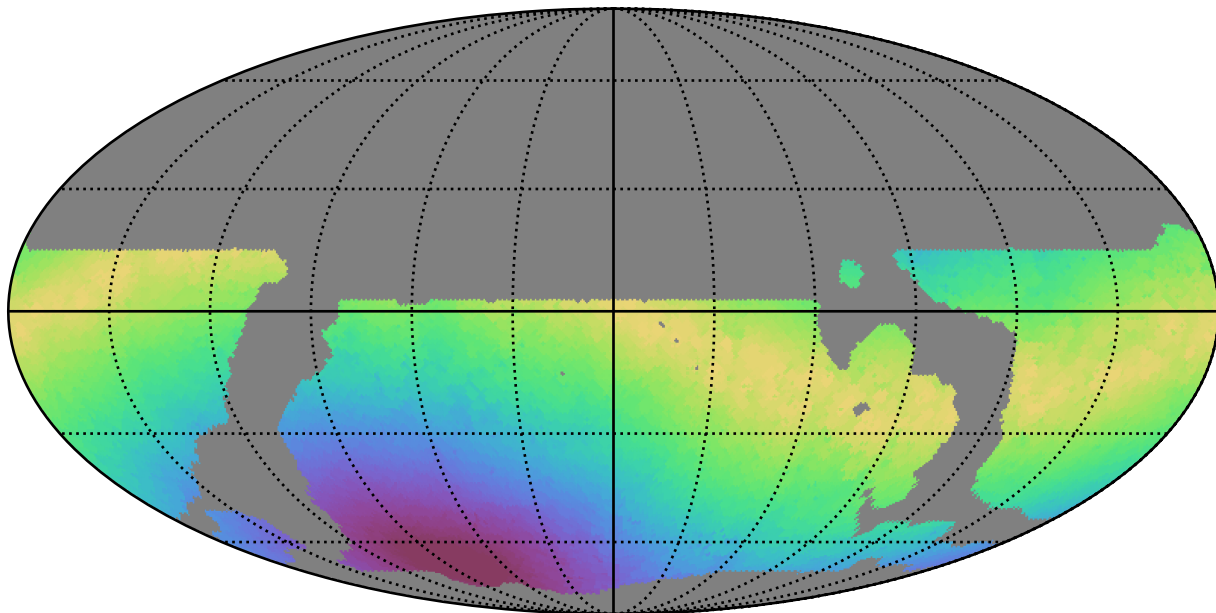
weather_cloudso16v3.4_10yrs WFD g band: Max moonDistance
