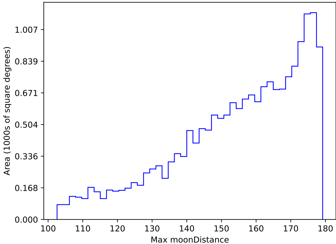
weather_cloudso16v3.4_10yrs WFD g band: Max moonDistance
