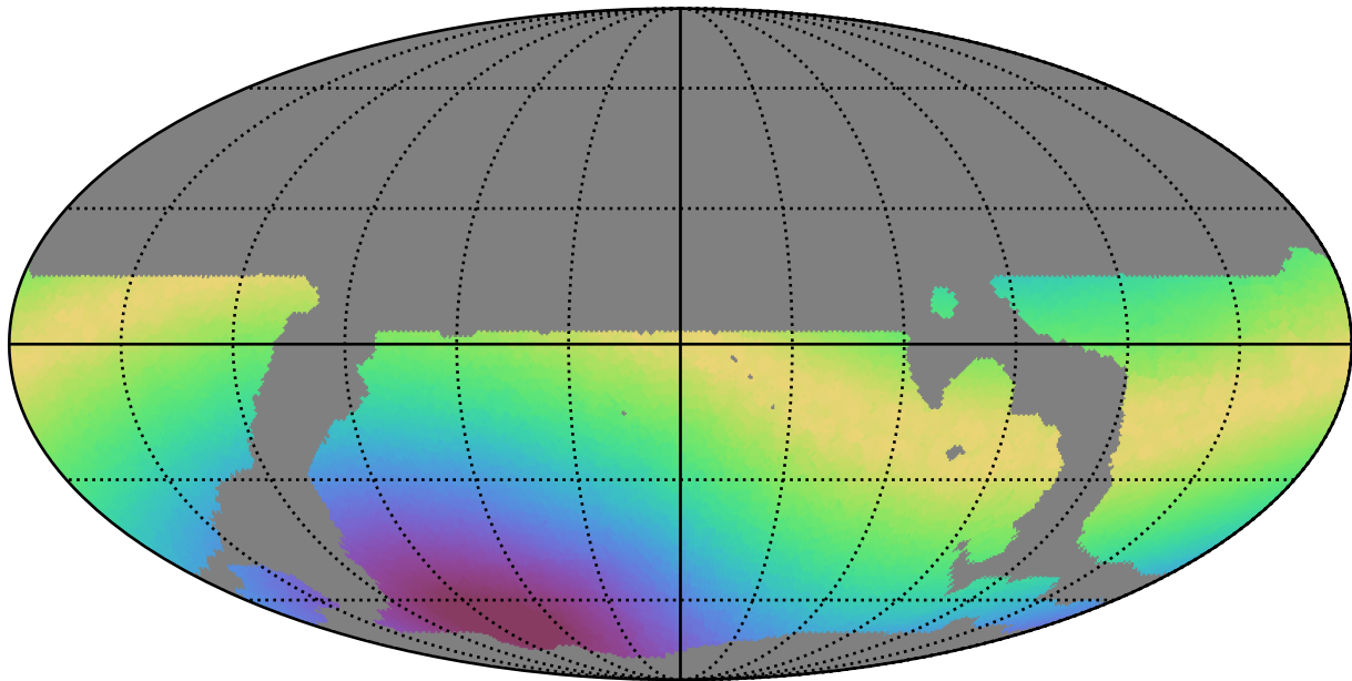
weather_cloudso16v3.4_10yrs WFD all bands: Max moonDistance
