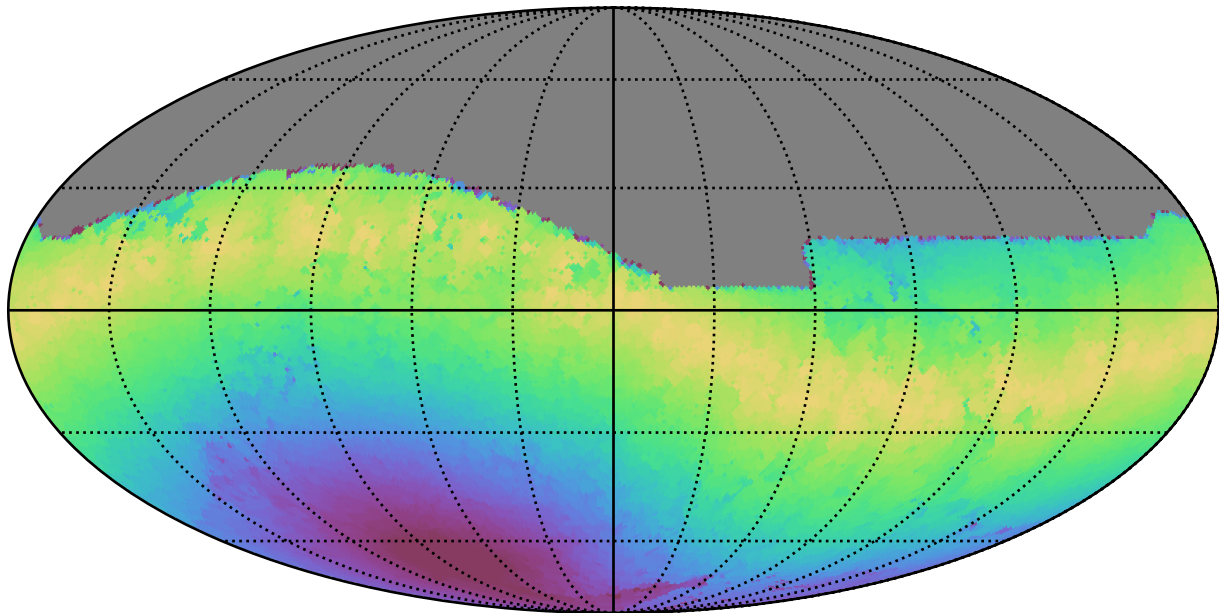
weather_cloudso16v3.4_10yrs All sky z band: Max moonDistance
