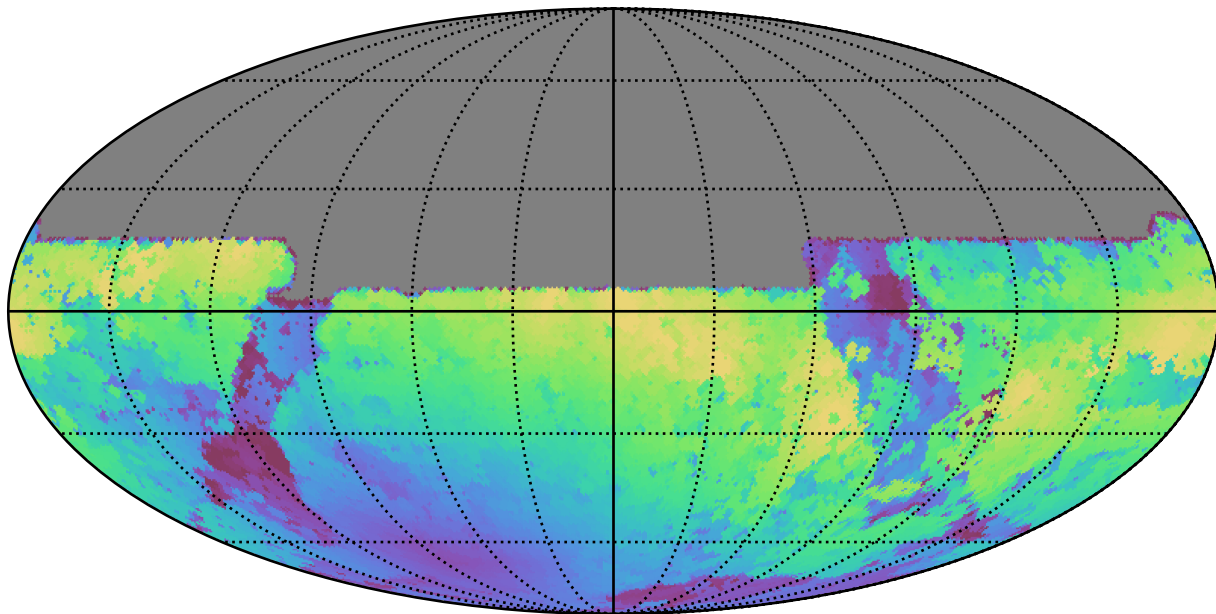
weather_cloudso16v3.4_10yrs All sky y band: Max moonDistance
