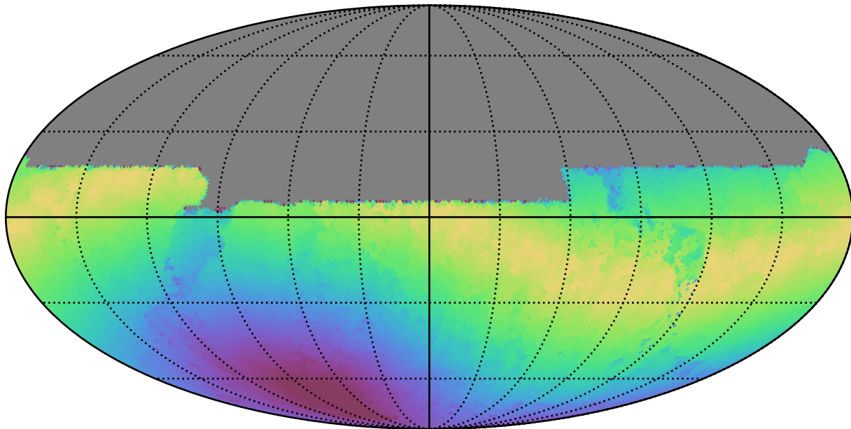
weather_cloudso16v3.4_10yrs All sky u band: Max moonDistance
