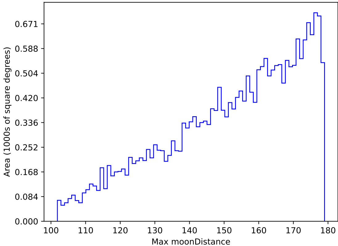
weather_cloudso16v3.4_10yrs All sky u band: Max moonDistance
