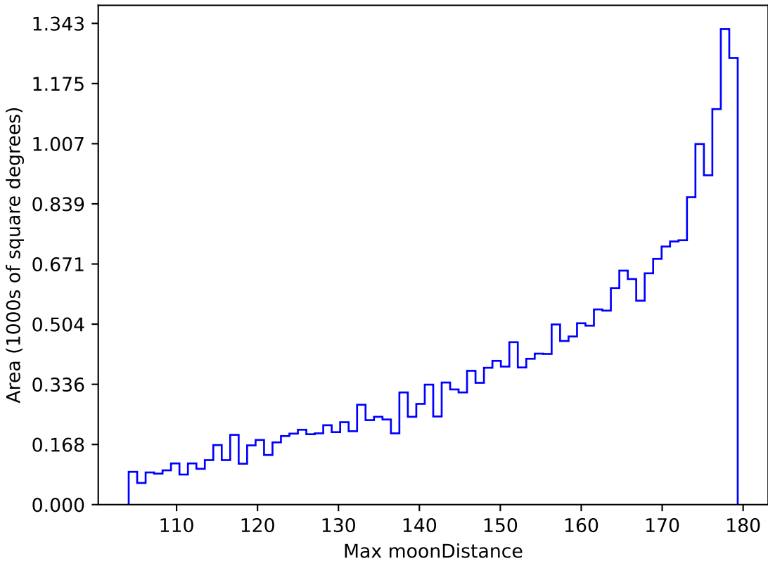
weather_cloudso16v3.4_10yrs All sky r band: Max moonDistance
