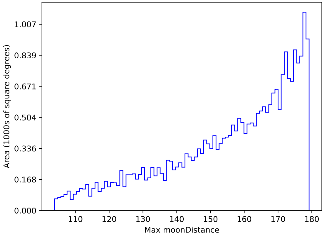
weather_cloudso16v3.4_10yrs All sky i band: Max moonDistance
