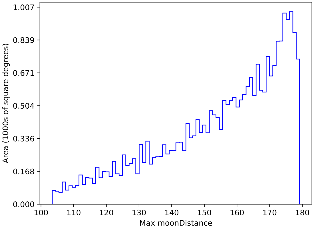
weather_cloudso16v3.4_10yrs All sky g band: Max moonDistance
