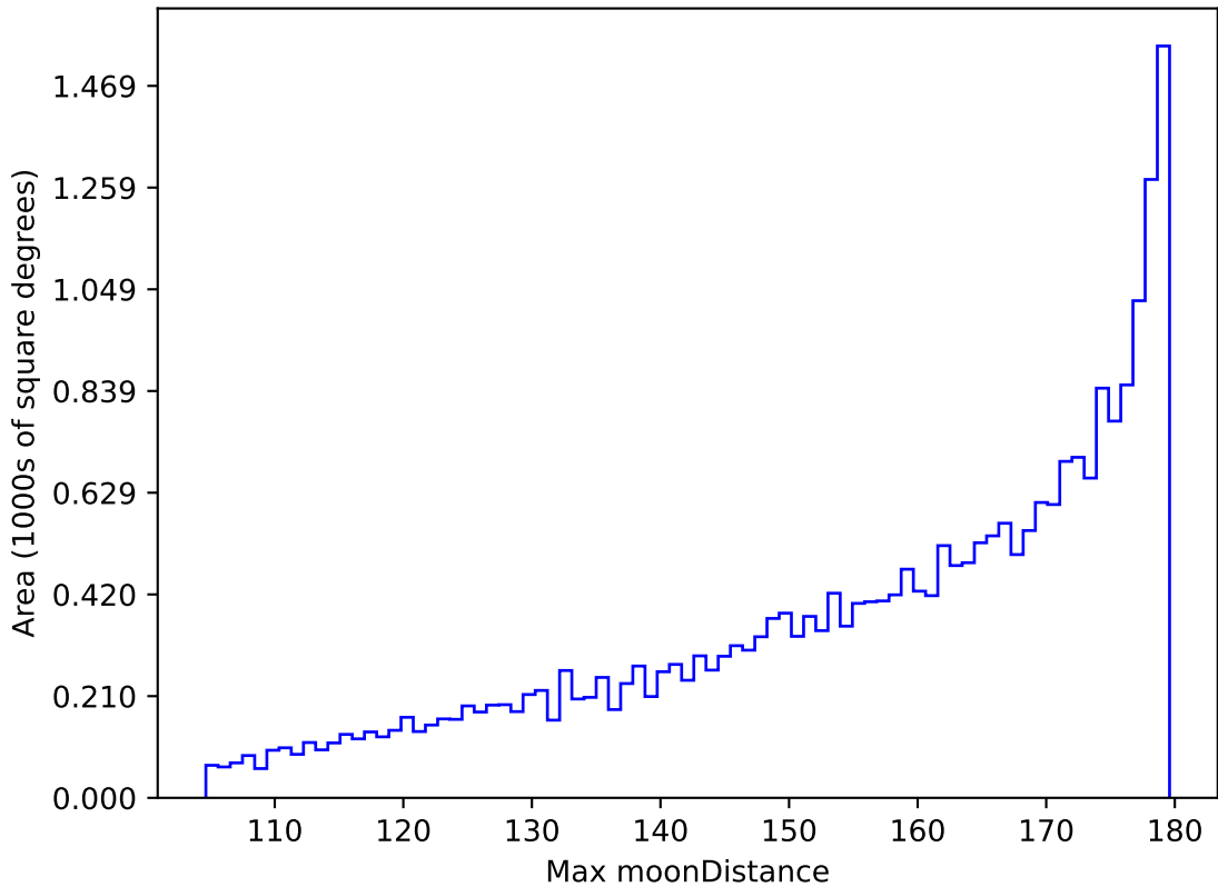
weather_cloudso16v3.4_10yrs All sky all bands: Max moonDistance
