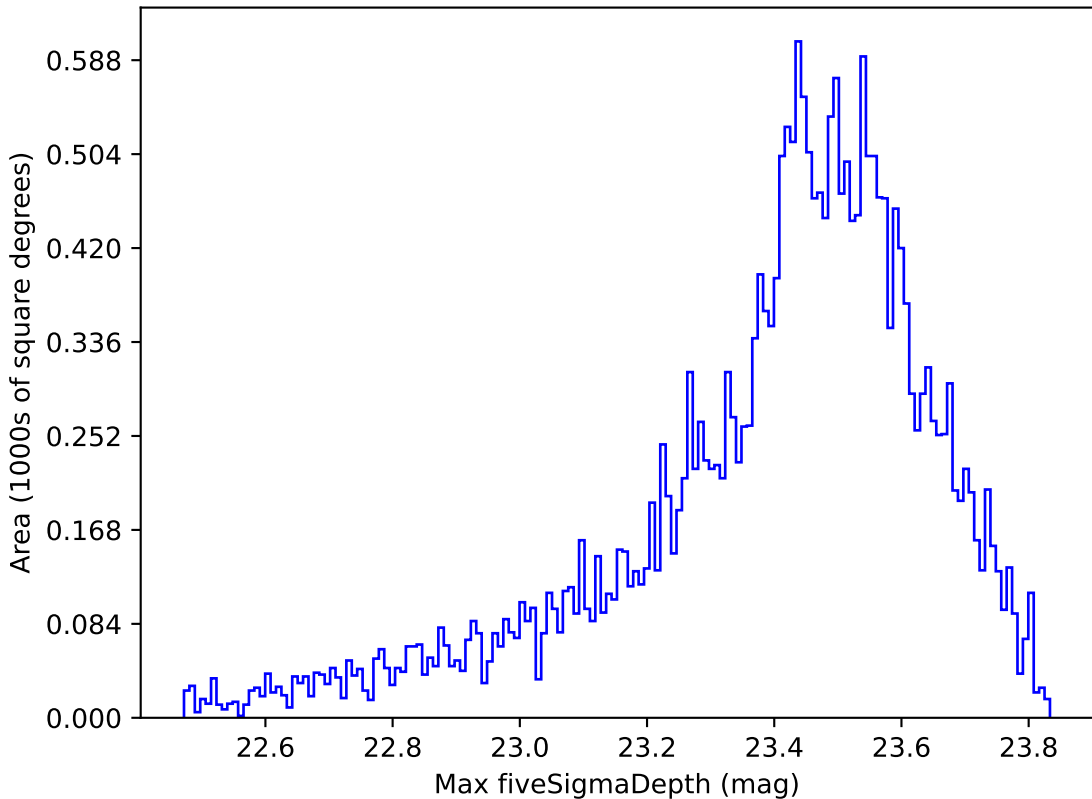
weather_cloudso16v3.4_10yrs Yr 1 z band: Max fiveSigmaDepth
