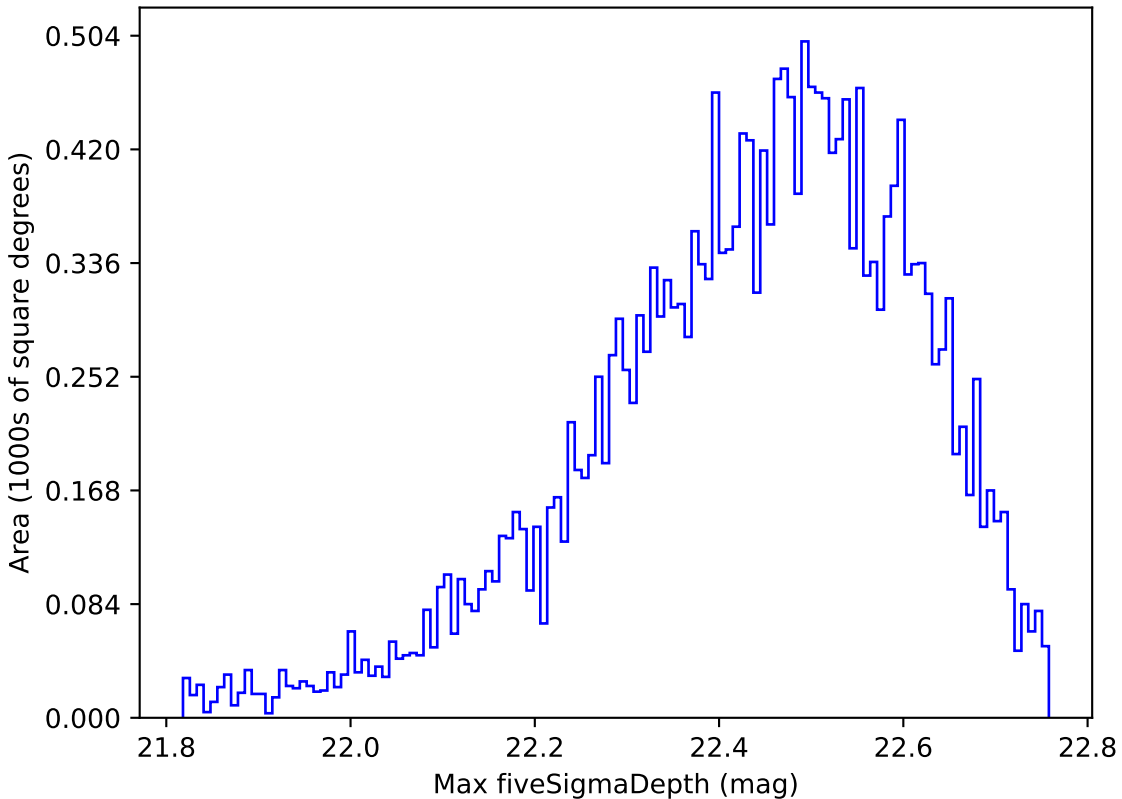
weather_cloudso16v3.4_10yrs Yr 1 y band: Max fiveSigmaDepth
