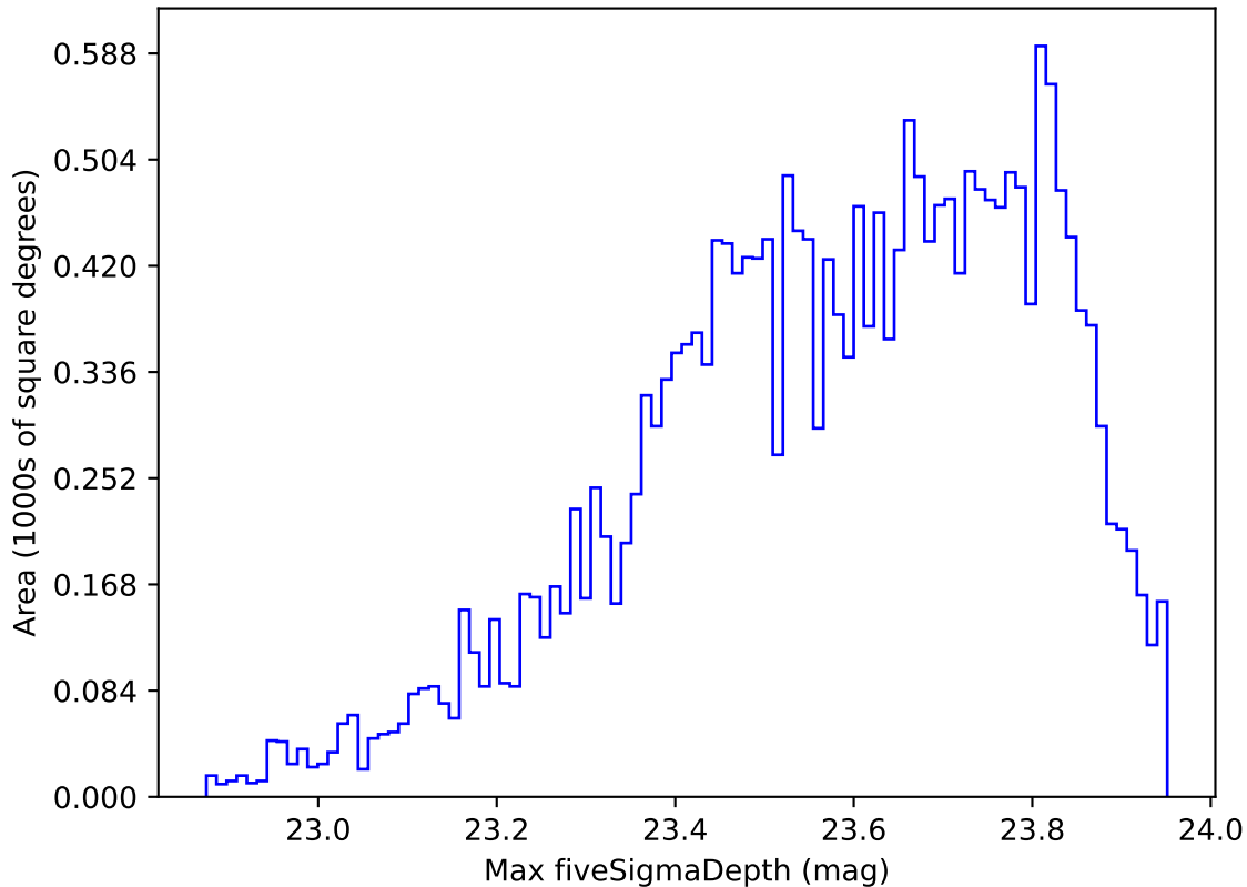
weather_cloudso16v3.4_10yrs Yr 1 u band: Max fiveSigmaDepth
