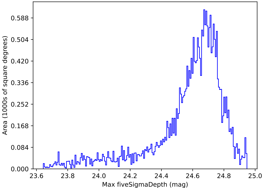
weather_cloudso16v3.4_10yrs Yr 1 r band: Max fiveSigmaDepth
