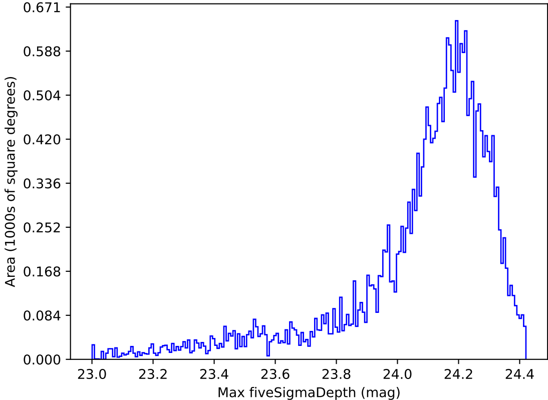
weather_cloudso16v3.4_10yrs Yr 1 i band: Max fiveSigmaDepth
