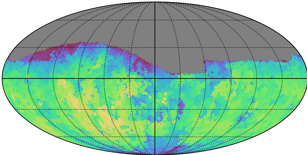
weather_cloudso16v3.4_10yrs Yr 1 g band: Max fiveSigmaDepth
