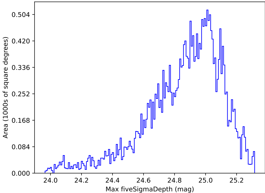
weather_cloudso16v3.4_10yrs Yr 1 g band: Max fiveSigmaDepth
