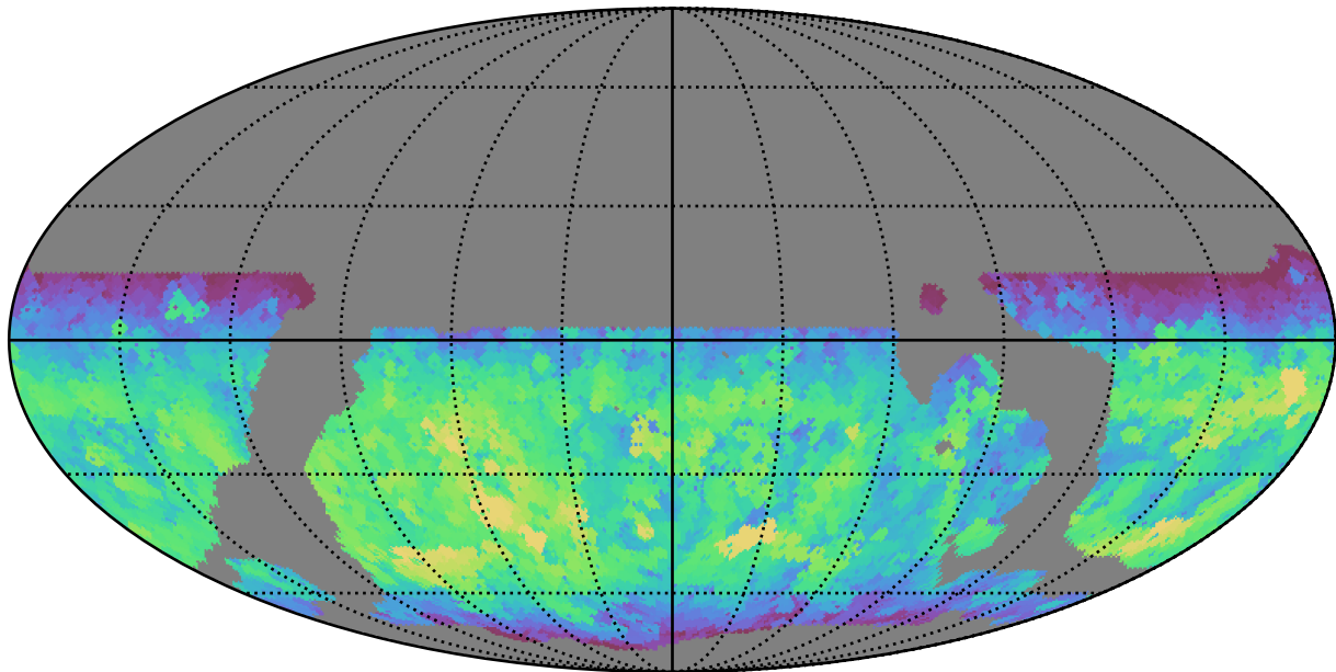
weather_cloudso16v3.4_10yrs WFD y band: Max fiveSigmaDepth
