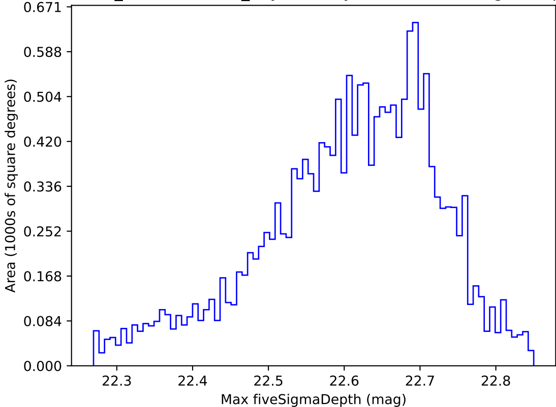
weather_cloudso16v3.4_10yrs WFD y band: Max fiveSigmaDepth
