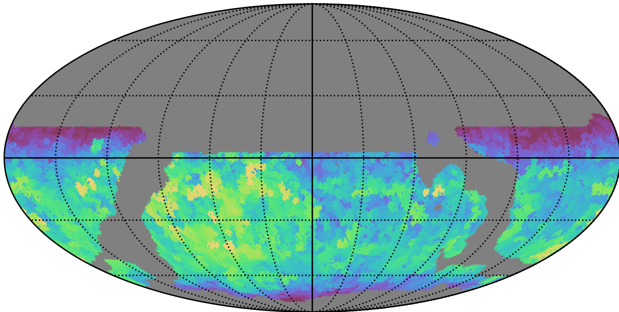
weather_cloudso16v3.4_10yrs WFD r band: Max fiveSigmaDepth
