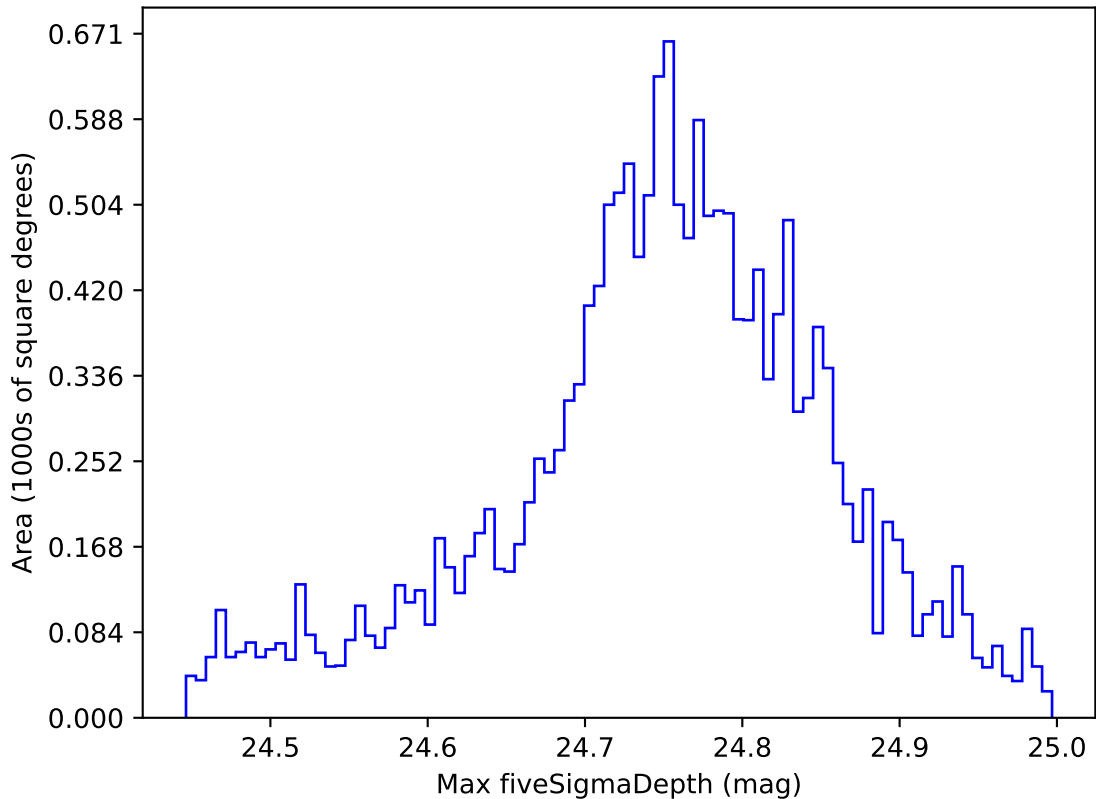
weather_cloudso16v3.4_10yrs WFD r band: Max fiveSigmaDepth
