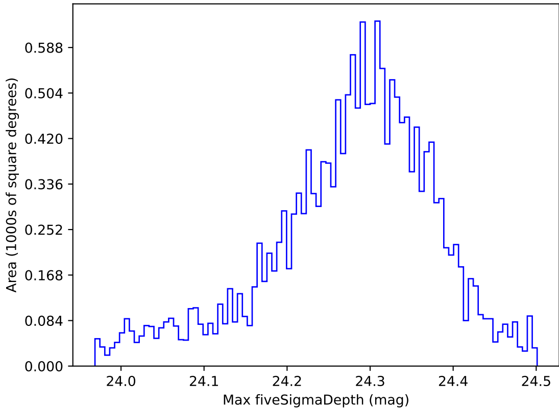
weather_cloudso16v3.4_10yrs WFD i band: Max fiveSigmaDepth
