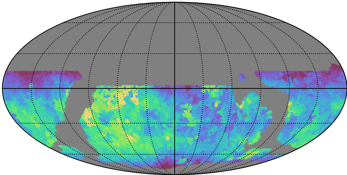
weather_cloudso16v3.4_10yrs WFD g band: Max fiveSigmaDepth
