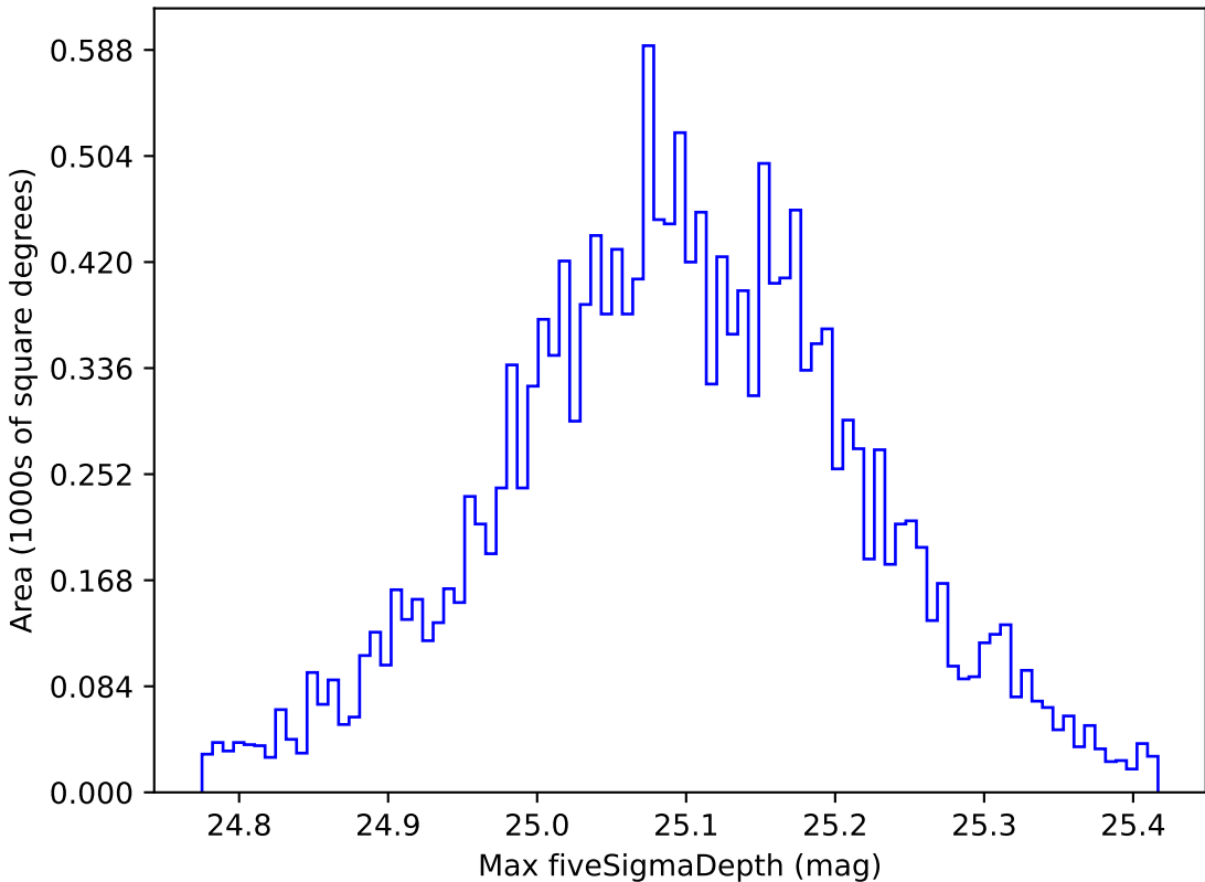
weather_cloudso16v3.4_10yrs WFD g band: Max fiveSigmaDepth
