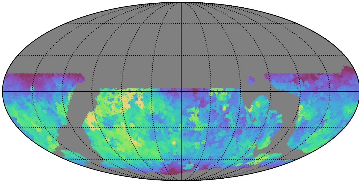
weather_cloudso16v3.4_10yrs WFD all bands: Max fiveSigmaDepth
