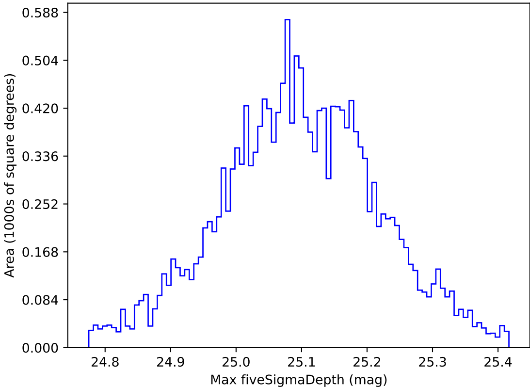
weather_cloudso16v3.4_10yrs WFD all bands: Max fiveSigmaDepth
