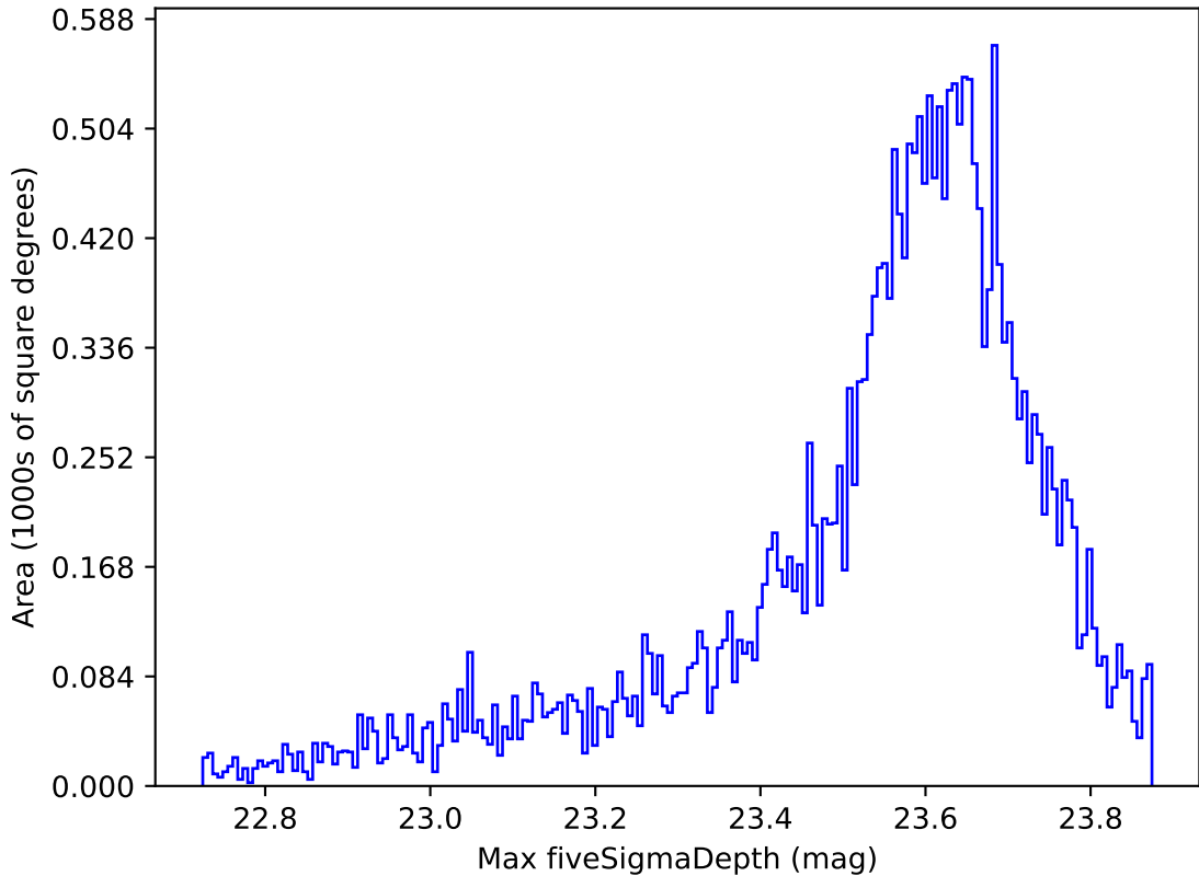
weather_cloudso16v3.4_10yrs All sky z band: Max fiveSigmaDepth
